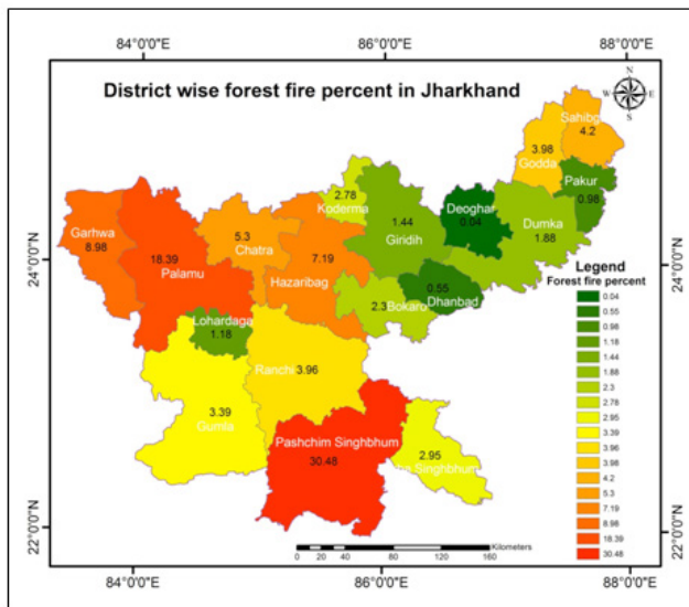
Figure 3. District wise forest fire % in Jharkhand.
