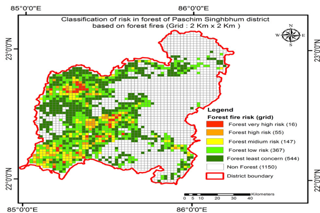
Figure 5. Grid based forest fire risk map of Paschim Singhbhum of Jharkhand.
