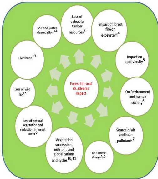
Figure 1. Forest fire and its adverse impact.
