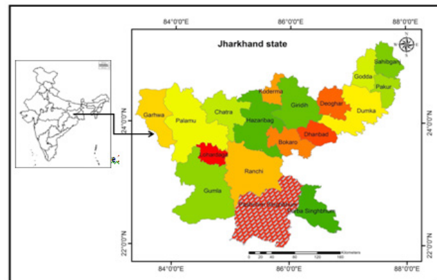
Figure 2. The location of the study area
