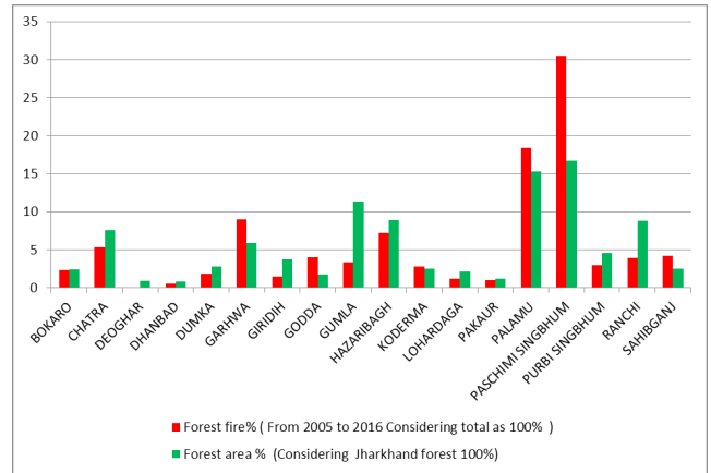
Figure 4. District wise forest fire % with respect to forest cover % of Jharkhand.
